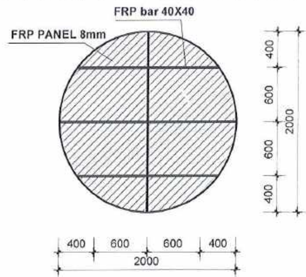
REINFORCING FOR BULKHEAD 2-6
